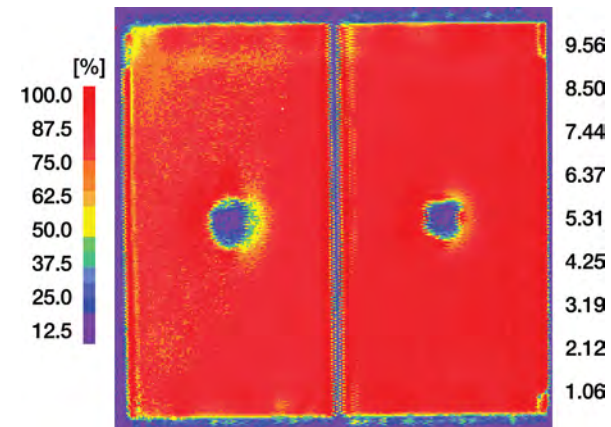
C-scan image of GILLFISTS core after impact
